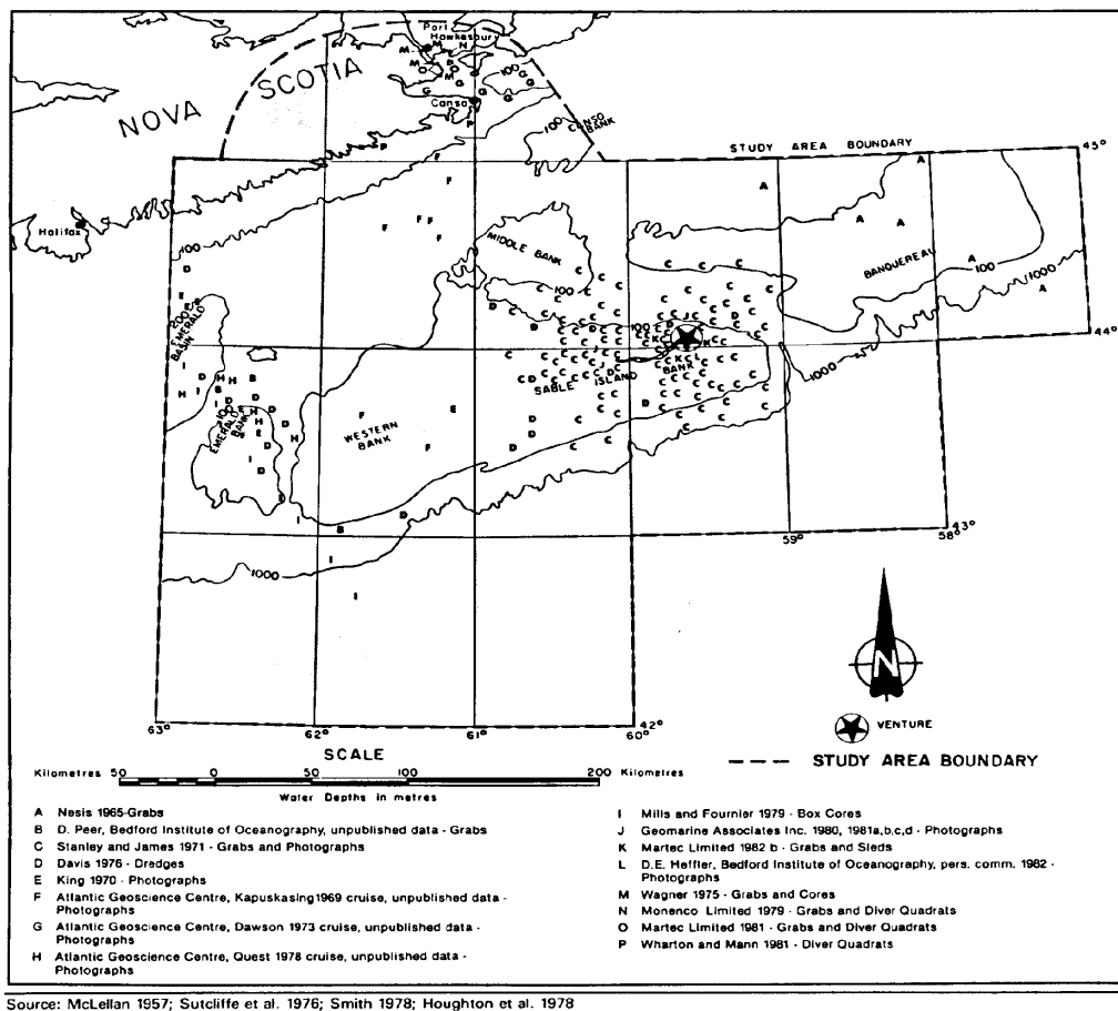
Figure 1. Summary of sources of information on benthic communities of the Scotian Shelf carried out pre-1983 (Mobil, 1983).
